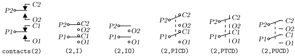
Figure 35: The contacts( poles, chars ) macro (drawing direction right).
