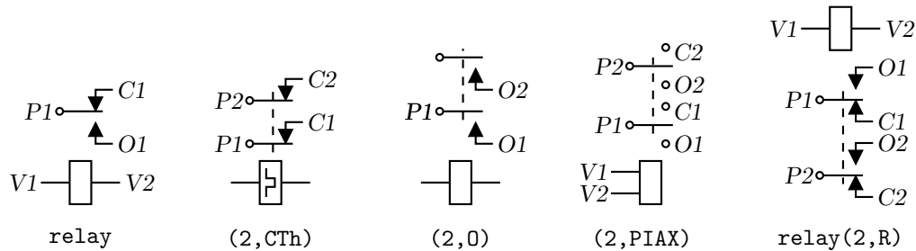
Figure 37: The relay( poles, chars ) macro (drawing direction right).
