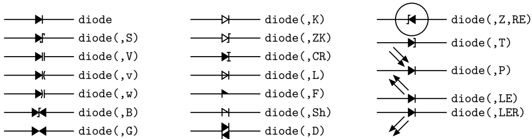
Figure 12: The macro diode( linespec ,B|CR|D|L|LE[R]|P[R]|S|T|V|v|w|Z|chars,[R][E]) . Appending K to the second argument draws an open arrowhead.
