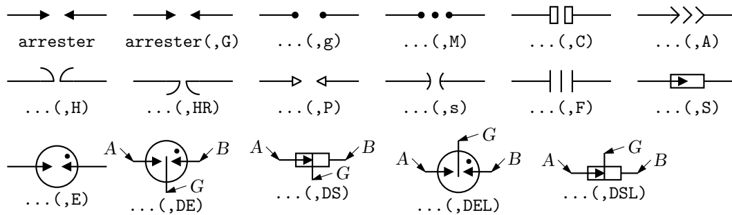
Figure 16: Variations of the arrester(linespec, chars, wid[:arrowhead ht], ht[:arrowhead wid]) macro. Putting D in argument 2 for the S or E configuration creates a 3-terminal composite element with terminals A, B, and G.
