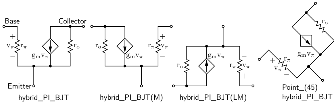
Figure 66: A composite element containing several basic elements
