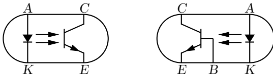
Figure 68: Showing opto and opto(BR) with defined labels.
