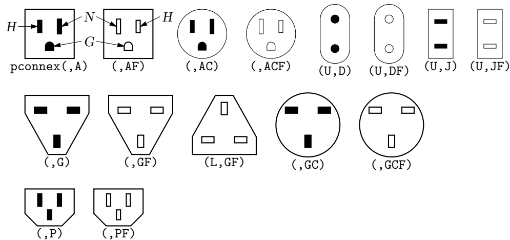
Figure 41: A small set of power connectors drawn by pconnex(R|L|U|D|degrees, chars) . Each connector has an internal H, N, and where applicable, a G shape.
