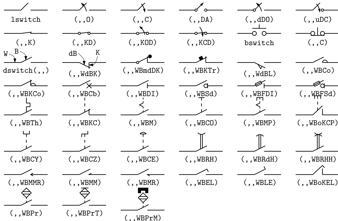
Figure 15: The switch(linespec,L|R,chars,L|B|D) macro is a wrapper for the macros lswitch(linespec,[L|R],[O|C][D][K][A]) , bswitch(linespec,[L|R],[O|C]) , and the many-optional dswitch(linespec,R,W[ud]B[K] chars) shown. The switch is drawn in the current drawing direction. A second-argument R produces a mirror image with respect to the drawing direction. The separately defined macros Proxim and Magn embellish switches in the second-last row.
