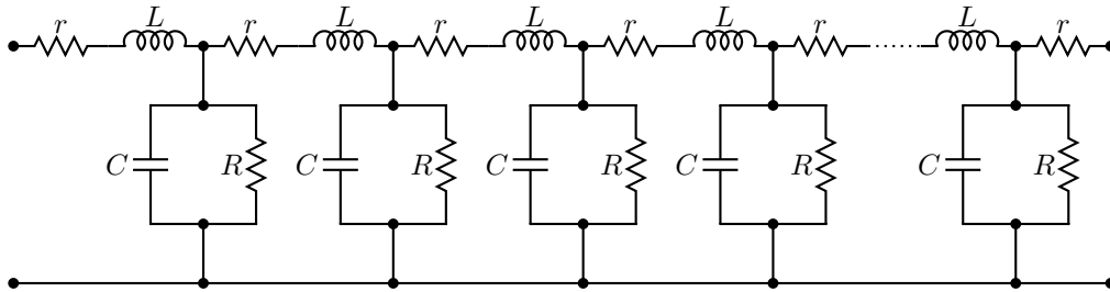
Figure 65: A lumped model of a transmission line, illustrating the use of custom macros.
