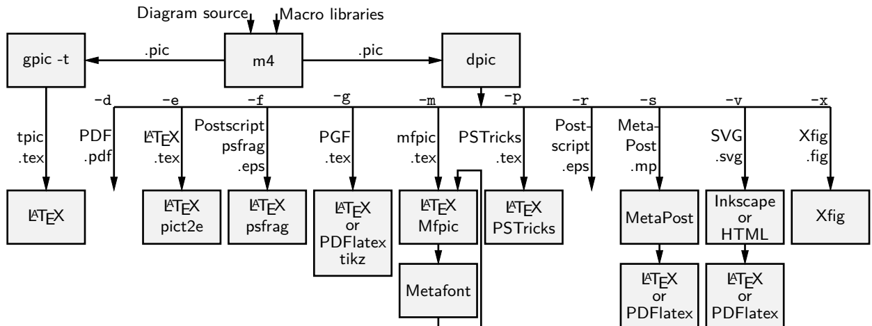
Figure 73: Output formats produced by gpict-t and dpic . SVG output can be read by Inkscape or used directly in web documents.
