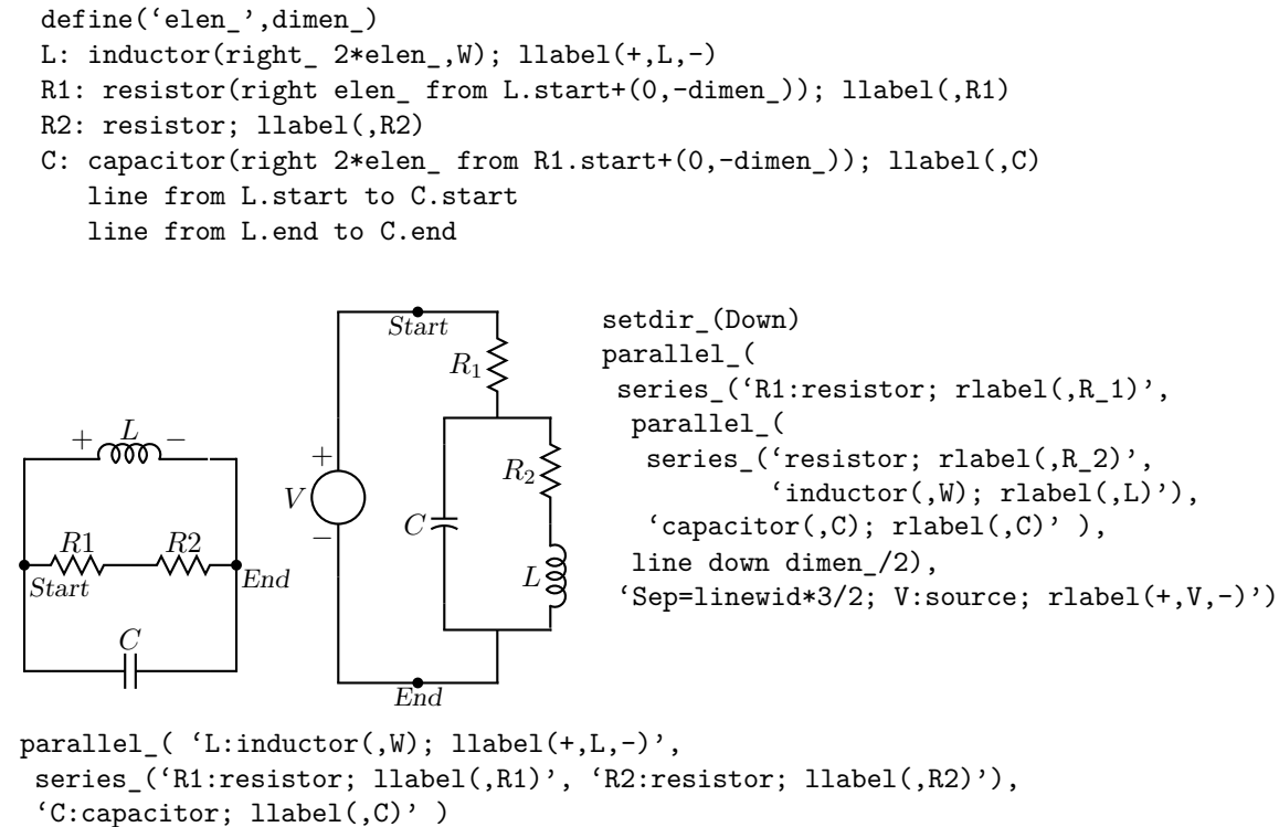
Figure 22: Illustrating the macros parallel_ and series_ , with Start and End points marked.
