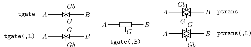
Figure 51: The tgate(linespec, [B] [R|L]) element, derived from a customized diode and ebox , and the ptrans(linespec, [R|L]) macro. These are not two-terminal elements, so the linespec argument defines the direction and length of the line from A to B but not the element position.
